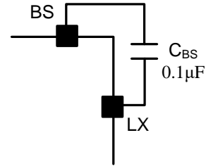
Fig 4. BS Capacitor Connection
