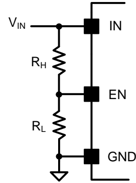
Fig 5. Adjusting Input UVLO
