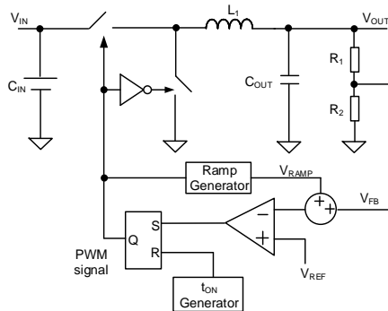
Fig 3. COT Architecture
