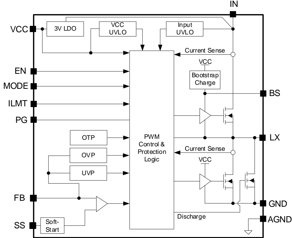
Figure2. Block Diagram
