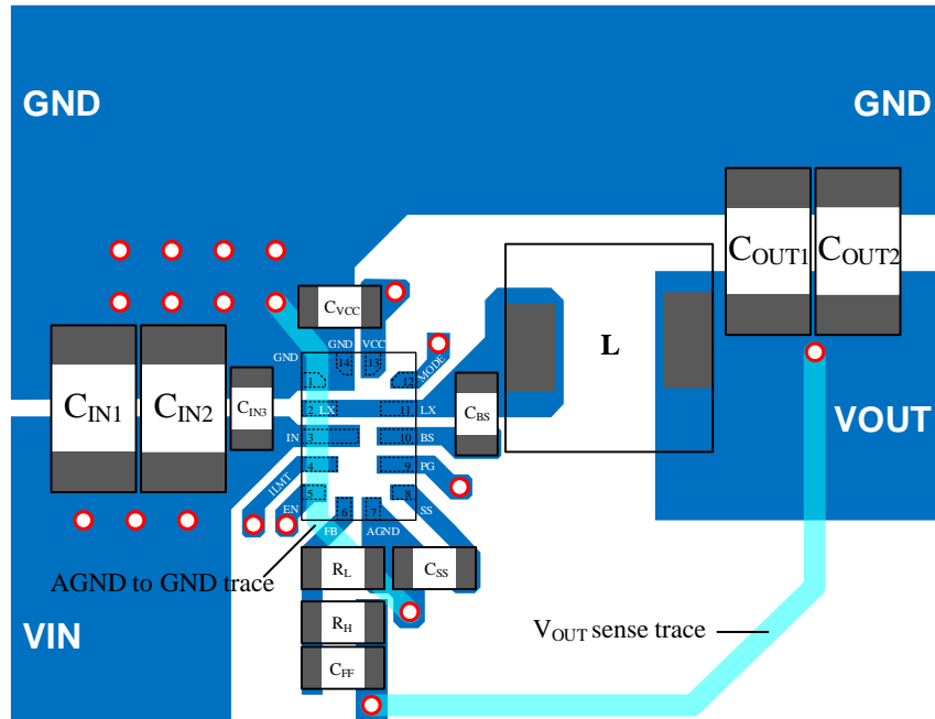
Fig.8 PCB Layout Suggestion
