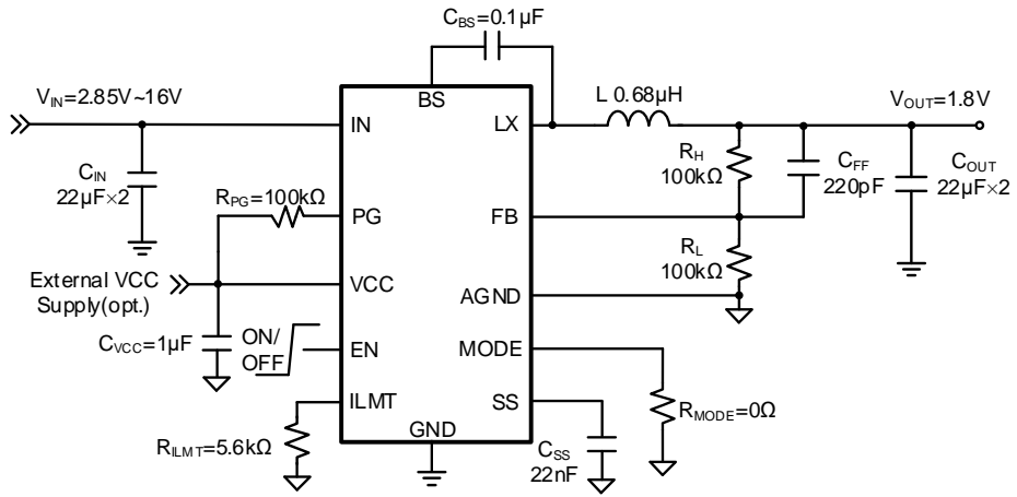
Figure1. Application Circuit
