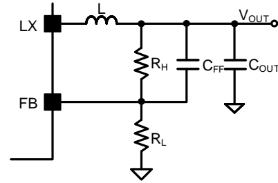
Fig 7. Feed-forward Capacitor
