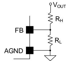
Fig 6. Feedback Resistor
