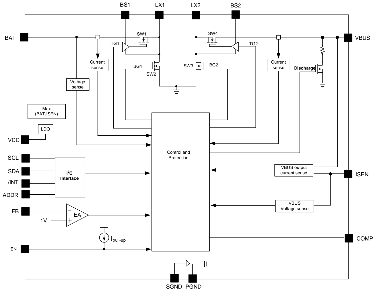
Figure.2 Block Diagram
