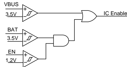
Figure6. Description of the IC Enable Function
