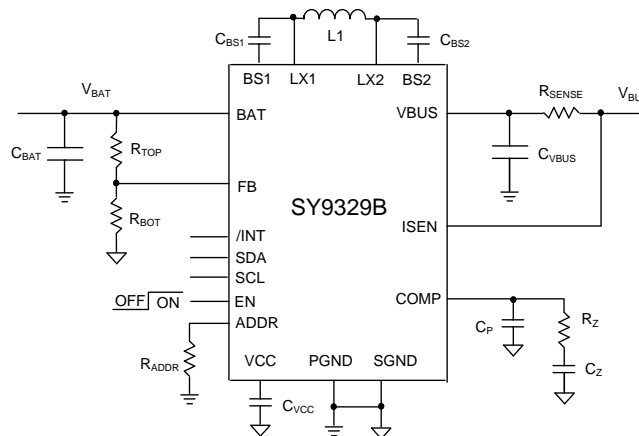
Figure1. Typical Schematic Diagram
